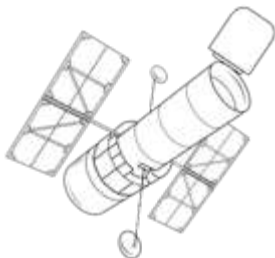
Hubble Telescope
